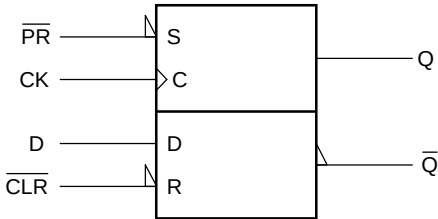
Logic Diagram
