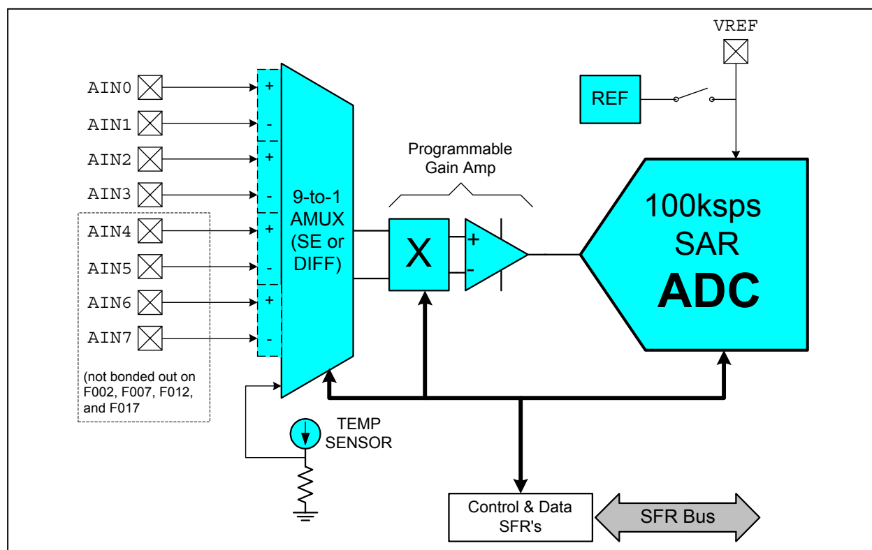
Figure 1.10. ADC Diagram
