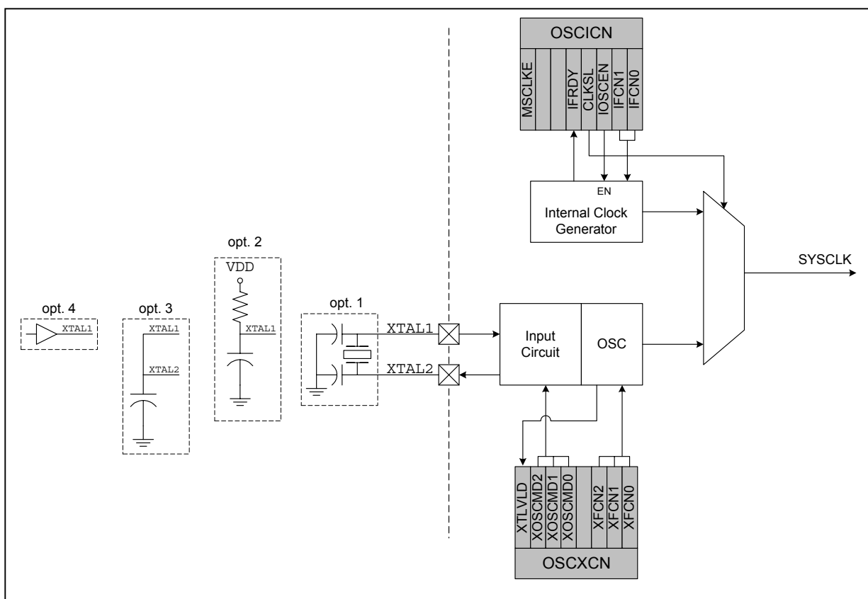
Figure 14.1. Oscillator Diagram
