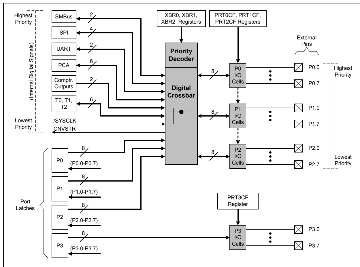
Figure 15.1. Port I/O Functional Block Diagram
