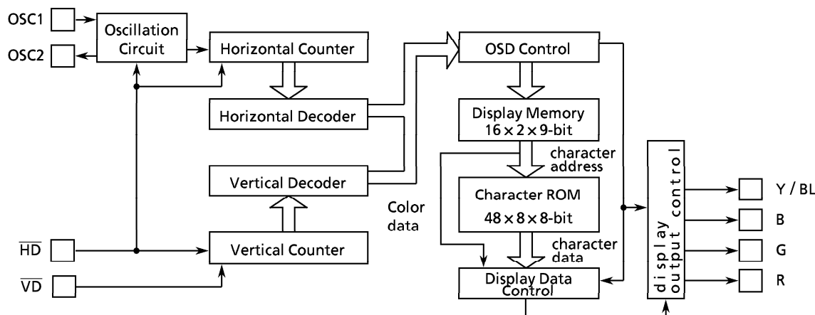
Figure 3-4. OSD Circuit
