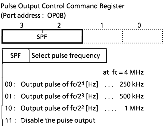
Figure 3-17. Pulse Output Command Register
