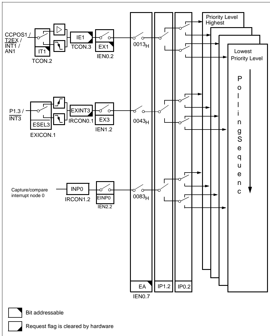
Figure 25 Interrupt Structure, Overview Part 2
