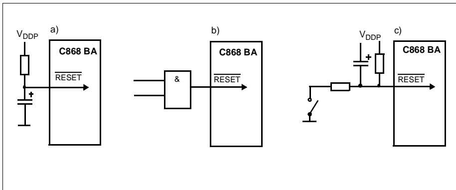
Figure 10 Reset Circuitries
