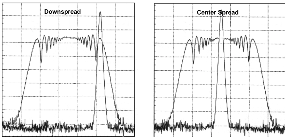
Figure 7. Spread Spectrum
