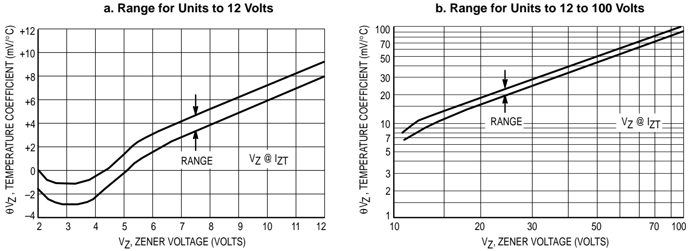
Figure 2. Temperature Coefficients
