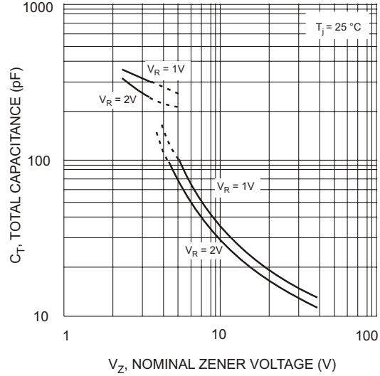
C_T , TOTAL CAPACITANCE (pF) V_Z , NOMINAL ZENER VOLTAGE (V) Fig. 4. Total Capacitance vs Nominal Zener Voltage
