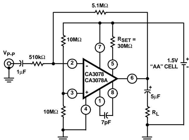
FIGURE 4. INVERTING 20dB AMPLIFIER CIRCUIT
