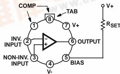
CA3078 (METAL CAN) TOP VIEW
