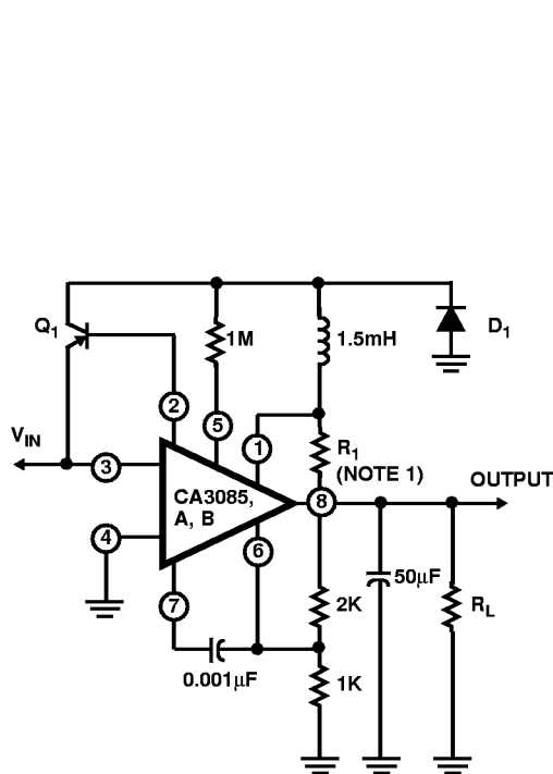
FIGURE 17. TYPICAL HIGH CURRENT VOLTAGE REGULATOR CIRCUIT
