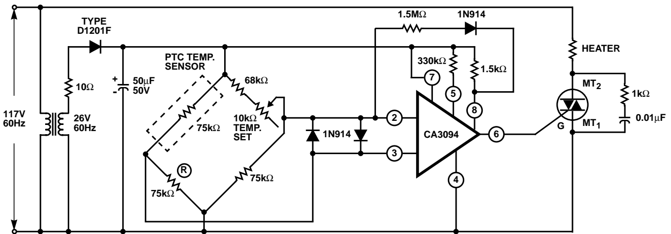
FIGURE 19. TEMPERATURE CONTROLLER
