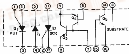
Fig. 1 — Schematic diagram of CA3097E.
