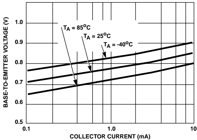
FIGURE 6. BASE-TO-EMITTER VOLTAGE vs COLLECTOR CURRENT
