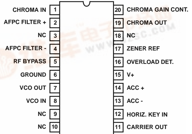
CA3126 (SOIC) TOP VIEW
