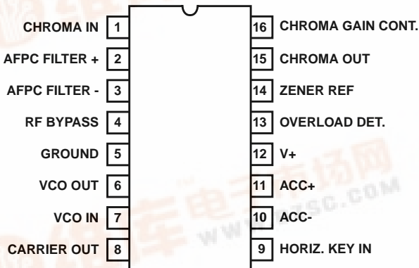
CA3126 (PDIP) TOP VIEW
