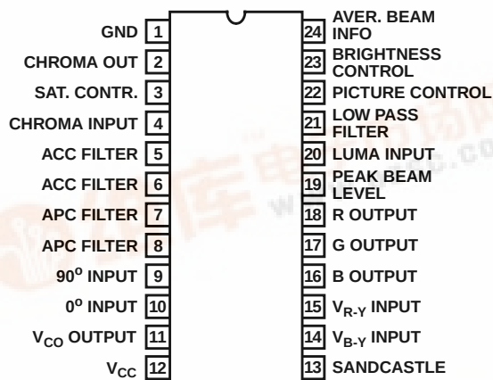
CA3194 (PDIP) TOP VIEW
