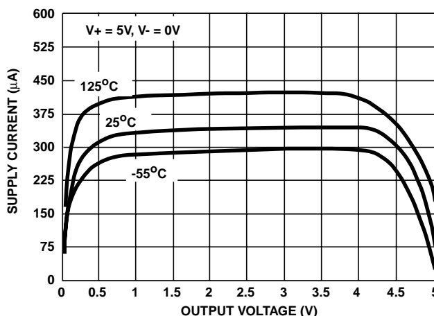
FIGURE 23. SUPPLY CURRENT vs OUTPUT VOLTAGE
