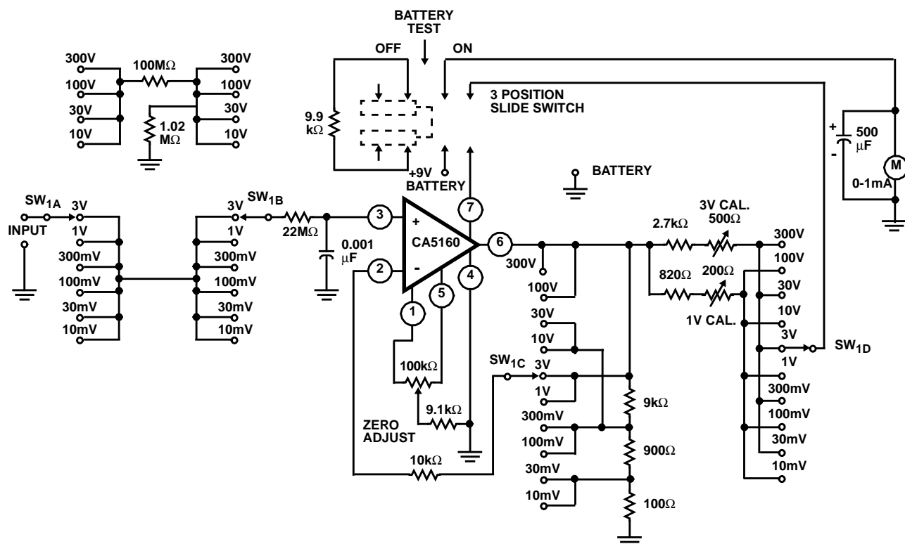
FIGURE 11. CA5160A HIGH INPUT RESISTANCE DC VOLTMETER
