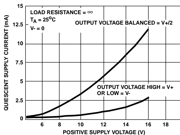
FIGURE 21. QUIESCENT SUPPLY CURRENT vs SUPPLY VOLTAGE
