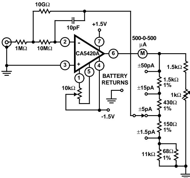
FIGURE 1. PICOAMMETER CIRCUIT
