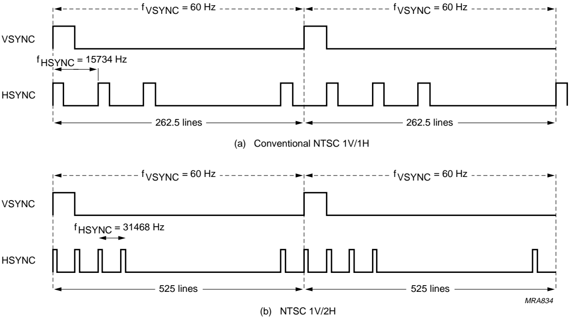
Fig.11 NTSC scan formats.
