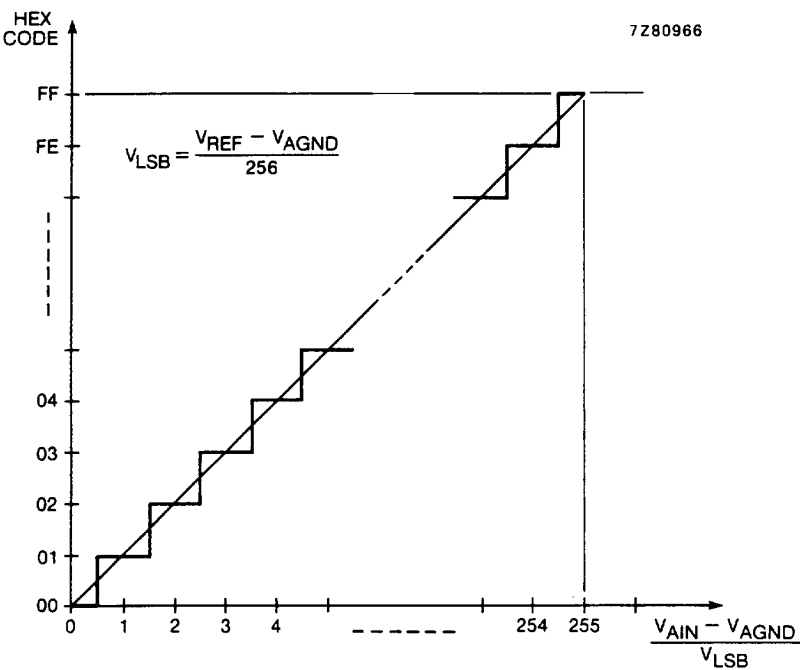
Fig.9 A/D conversion characteristics of single-ended inputs.
