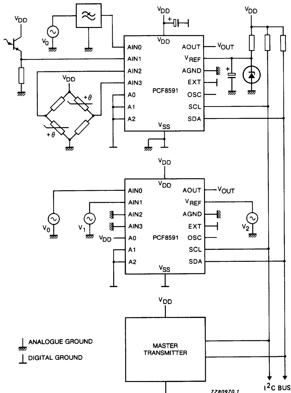
Fig.20 Application diagram.
