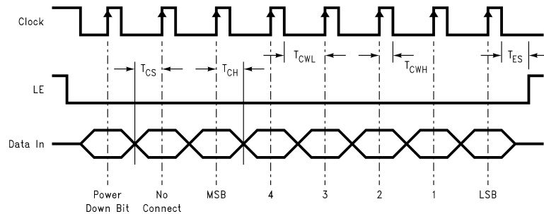
FIGURE 2. MICROWIRE Interface Timing Diagram
