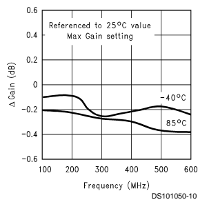
Gain Change Over Temperature vs. Frequency
