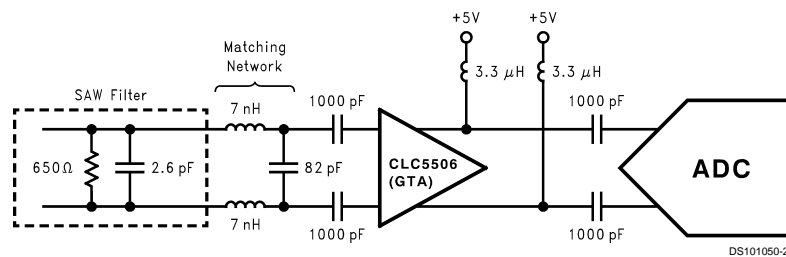
FIGURE 4. Narrow band design example with balanced SAW filter and ADC
