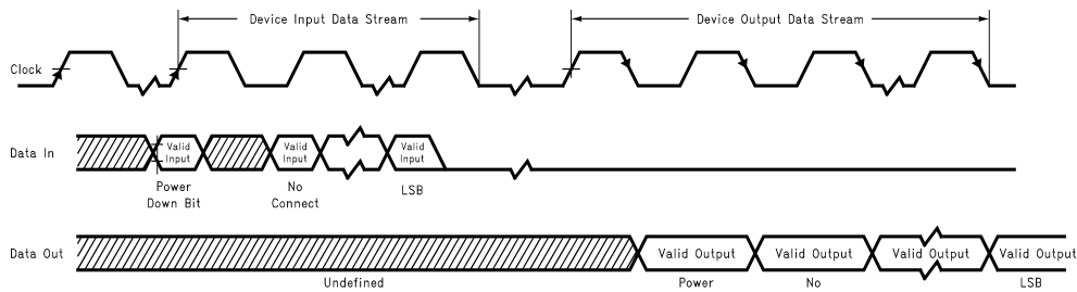
FIGURE 3. MICROWIRE Interface Serial Data Out Timing
