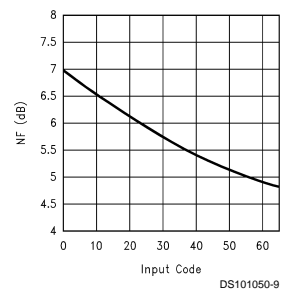
Noise Figure vs. Input Code
