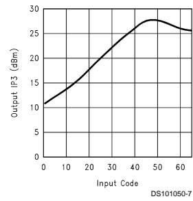
Output 3rd Order Intercept vs. Input Code
