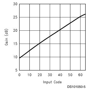
Gain vs. Input Code
