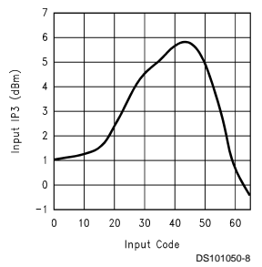
Input 3rd Order Intercept vs. Input Code
