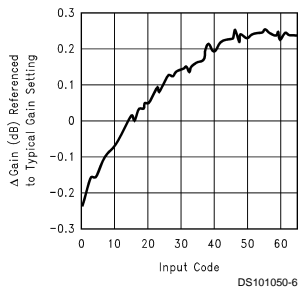
Gain Error vs. Input Code
