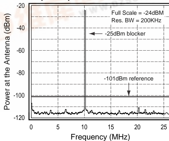
Output Response with GSM 1800 Blocker
