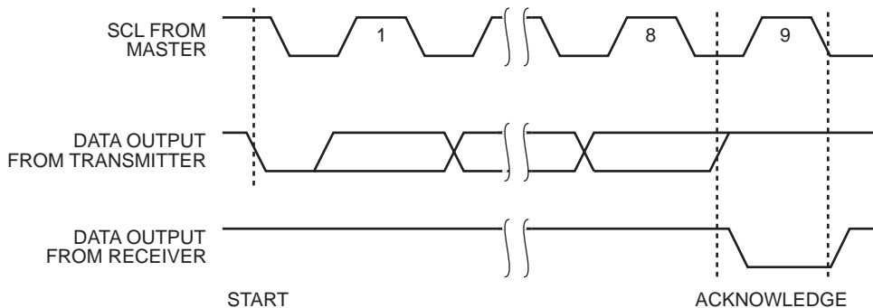
Figure 6. Acknowledge Timing
