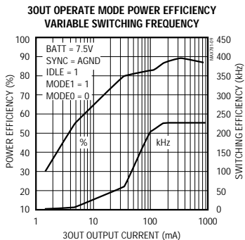
Typical Operating Characteristics (continued) (T A = +25°C, unless otherwise noted.)
