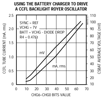
Typical Operating Characteristics (continued) (T A = +25°C, unless otherwise noted.)
