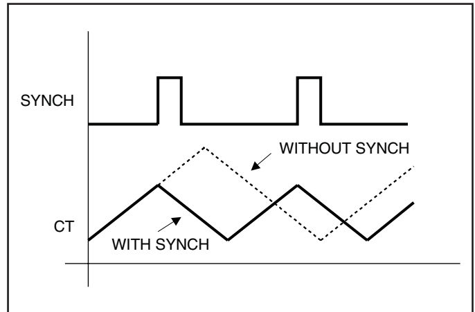
Figure 3. Synchronized and unsynchronized oscillator waveforms.
