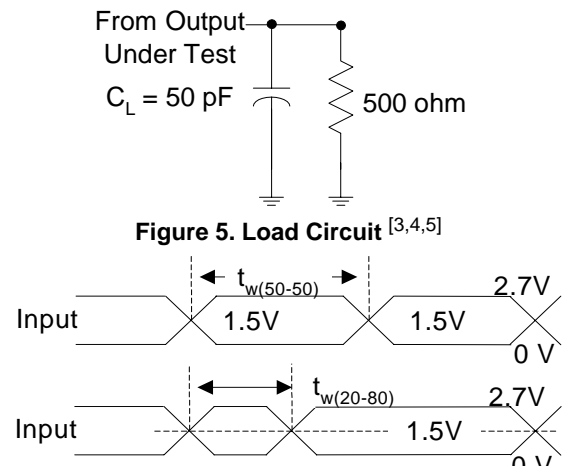
Figure 6. Voltage Waveforms–Pulse Duration [6]
