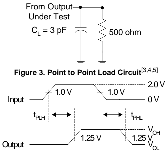
Figure 4. Voltage Waveforms–Propagation Delay Times [4]
