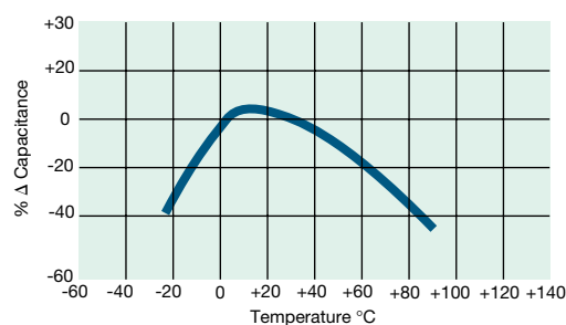
Temperature Coefficient
