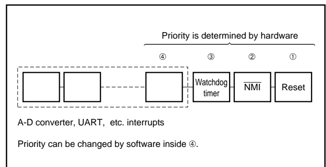
Fig. 36 Interrupt priority
