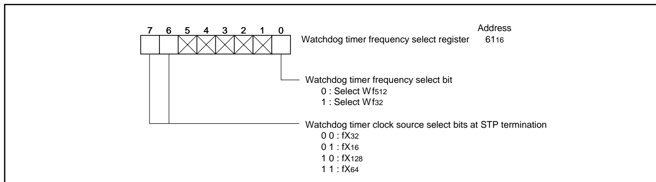
Fig. 102 Bit configuration of watchdog timer frequency select register
