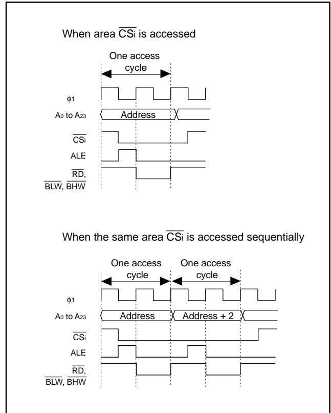
Fig. 27 Chip select output waveform example
