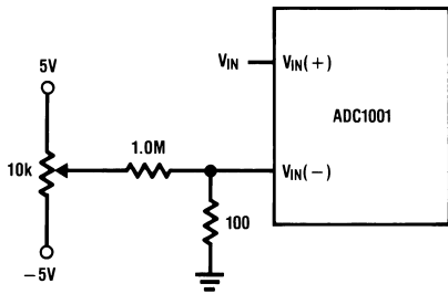
FIGURE 1. Zero Adjust Circuit
