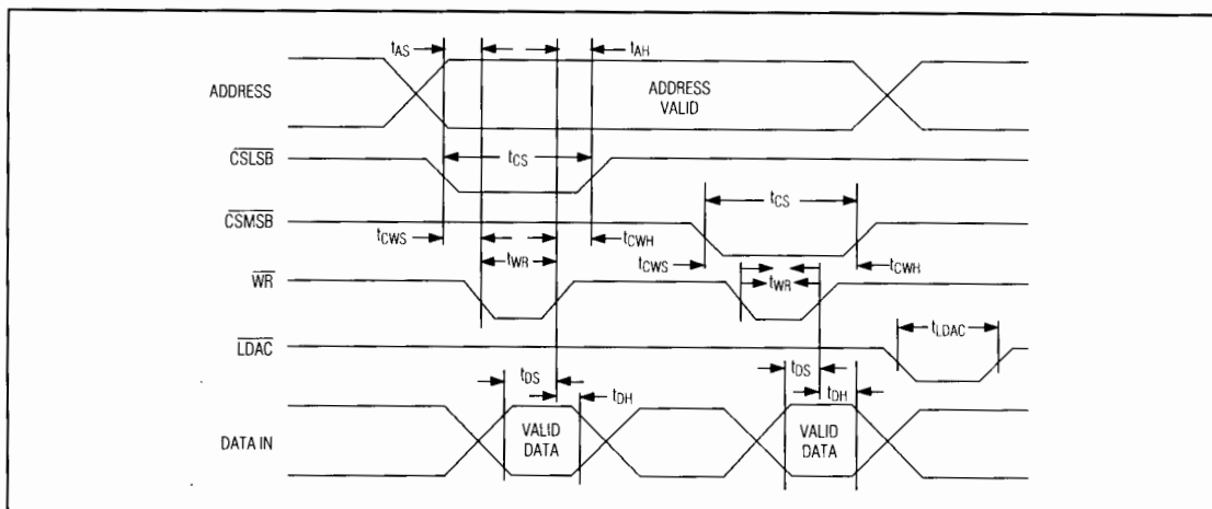
Figure 3. Write-Cycle Timing
