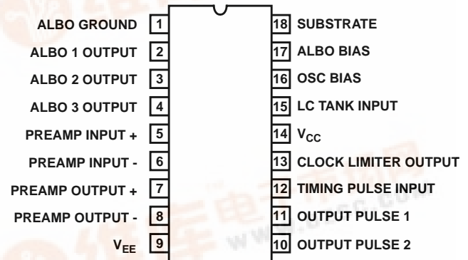
CD22301 (PDIP) TOP VIEW
