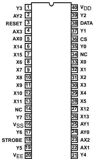
CD22M3494E (PDIP) TOP VIEW
