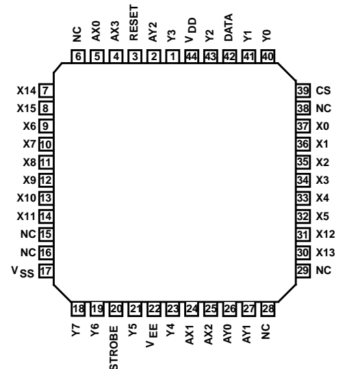
CD22M3494SQ (PLCC) (SGS LEAD COMPATIBLE) TOP VIEW
