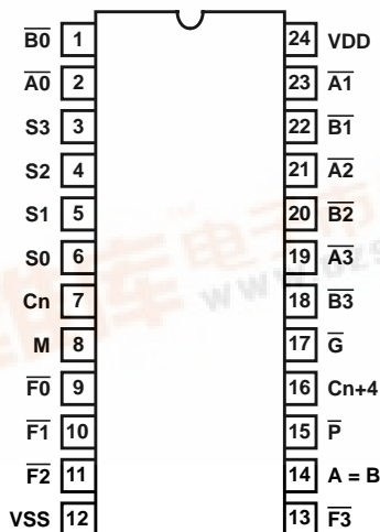
CD40181BMS ACTIVE-LOW DATA TOP VIEW
