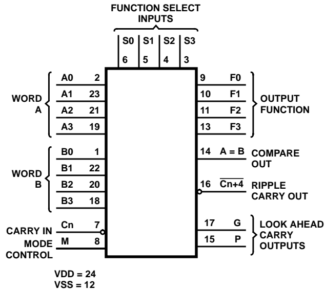
ACTIVE-HIGH DATA
