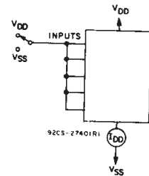
Fig. 15 - Quiescent-current test circuit.
