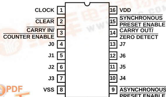
CD40102BMS, CD40130BMS TOP VIEW
