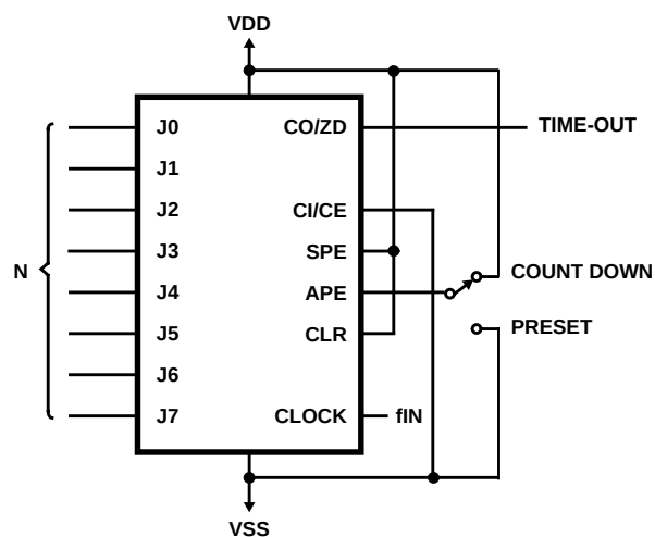
FIGURE 14. PROGRAMMABLE TIMER
