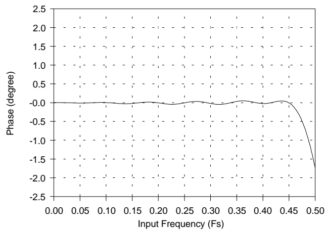
Figure 17. DAC Phase Response.
