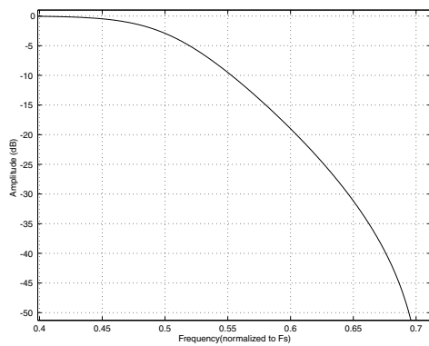
Figure 54. QSM Transition Band (detail)
