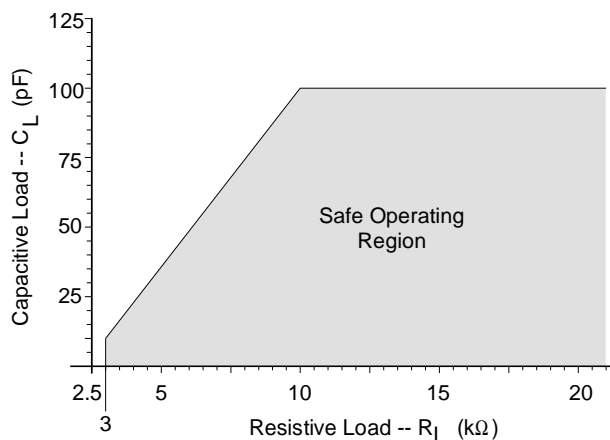
Figure 3. Maximum Loading
