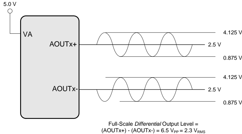
Figure 13. Full-Scale Output
