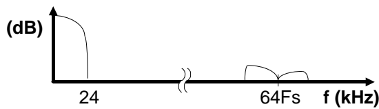
Figure 25. Spectrum After Switched-Capacitor Filter
