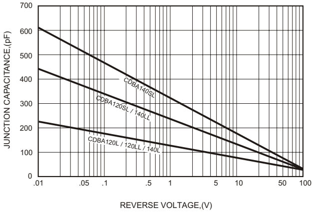
FIG.3-TYPICAL JUNCTION CAPACITANCE
