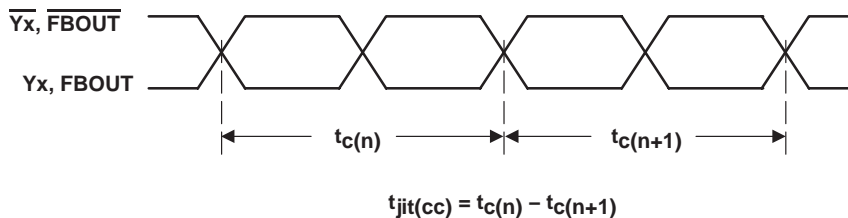
Figure 3. Cycle-to-Cycle Jitter
