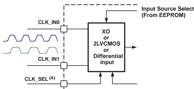
Figure 16. LVCMOS Clock Input Circuitry
