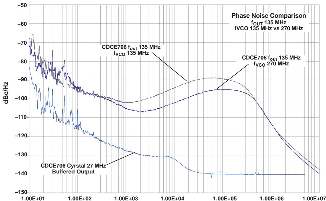
Figure 32. Phase Noise Characteristic - f_{\text{offset}} - Hz
