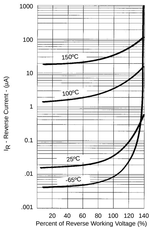
FIGURE 3 Typical Reverse Current vs Percent of Reverse Working Voltage
