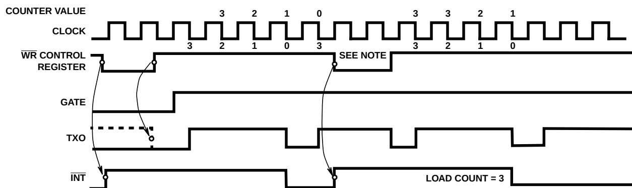
FIGURE 2. TIMEOUT STROBE (MODE 2) TIMING WAVEFORMS
