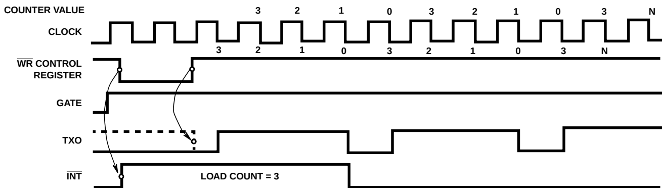
FIGURE 4. RATE GENERATORS (MODE 4) TIMING WAVEFORMS
