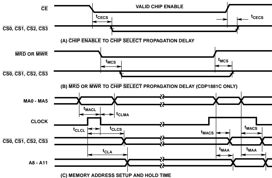
FIGURE 3. TIMING WAVEFORMS
