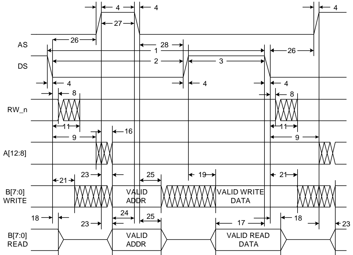
Figure 19. Bus Timing
