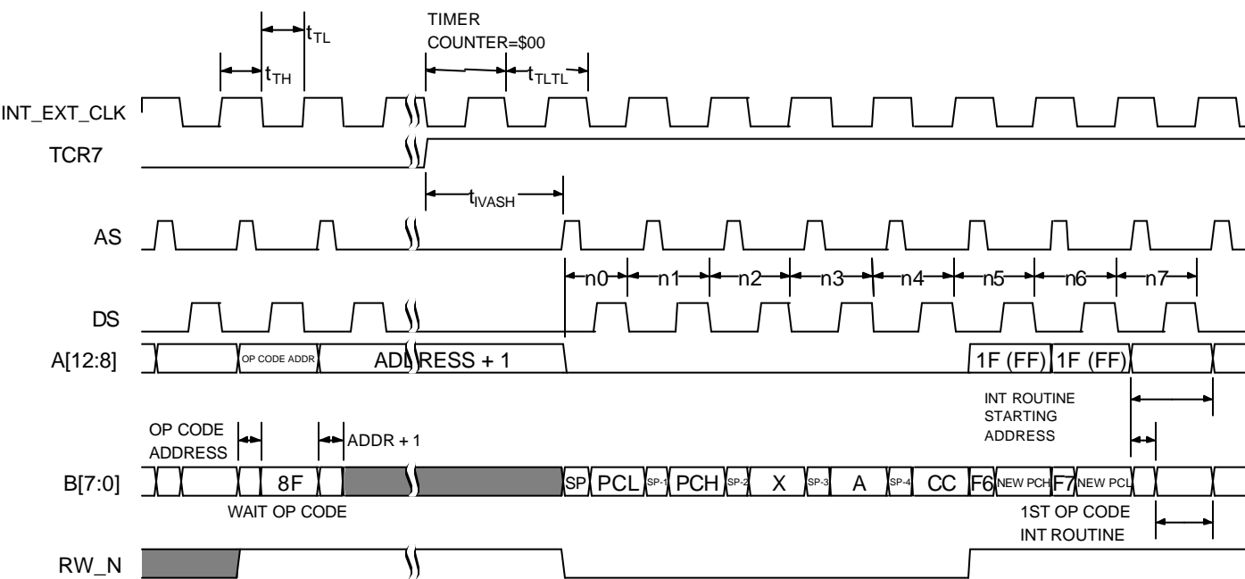
Figure 17. Timer Interrupt After WAIT Instruction Timing
