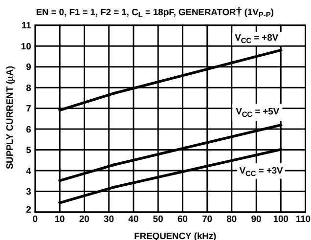
FIGURE 18. DISABLE SUPPLY CURRENT vs FREQUENCY
