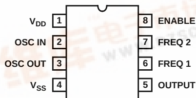
CDP6872 (PDIP, SOIC) TOP VIEW
