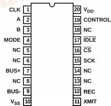
CD68HC68S1 (SOIC) TOP VIEW
