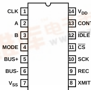
CD68HC68S1 (PDIP) TOP VIEW
