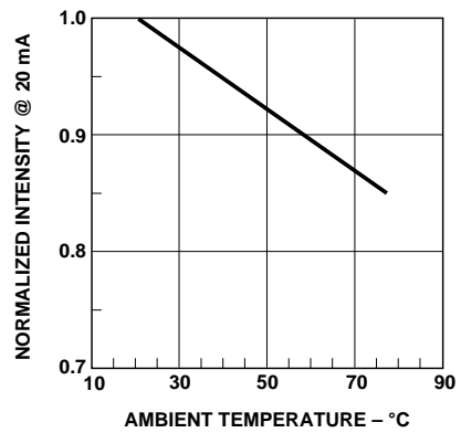
Figure 8. Normalized Intensity vs. Temperature.
