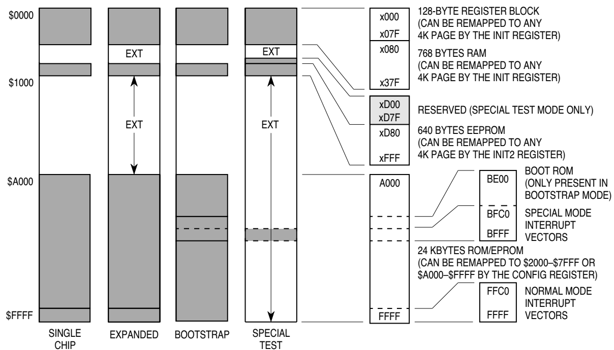
Figure 4 Memory Map
