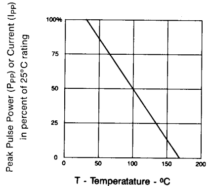
FIGURE 3 DERATING CURVE
