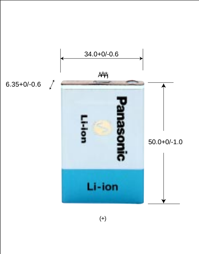
External Dimensions (mm) *2
