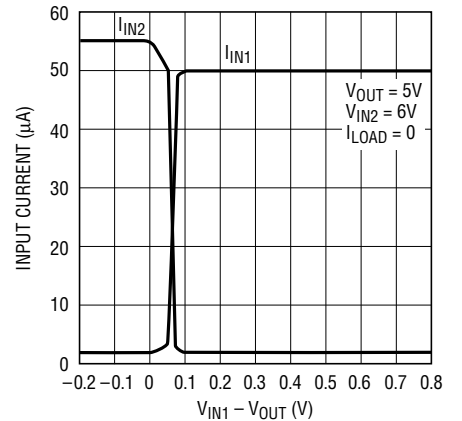
Input Current
